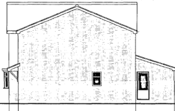
SIDE ELEVATION 'B' - EXISTING (1:100)
