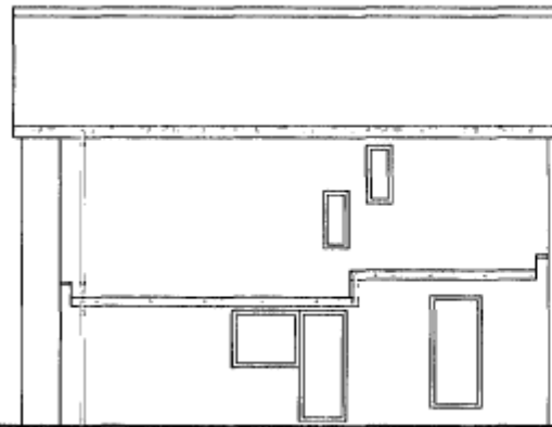
SIDE ELEVATION 'B' - EXISTING (1:100)
